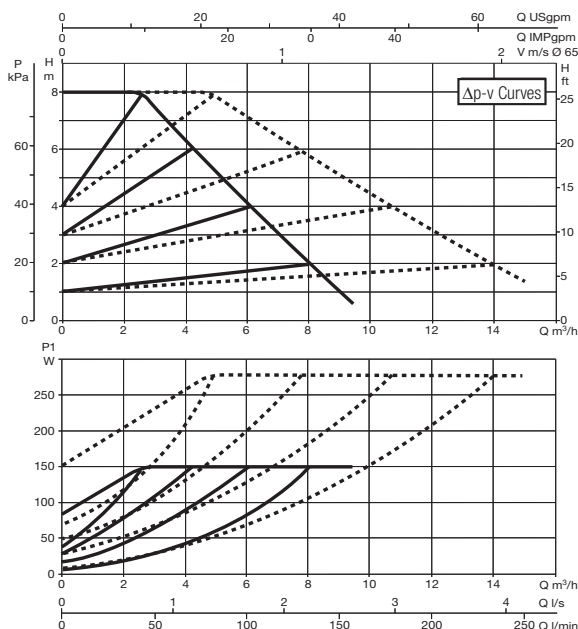
EVOPLUS D 80/220.32 M
