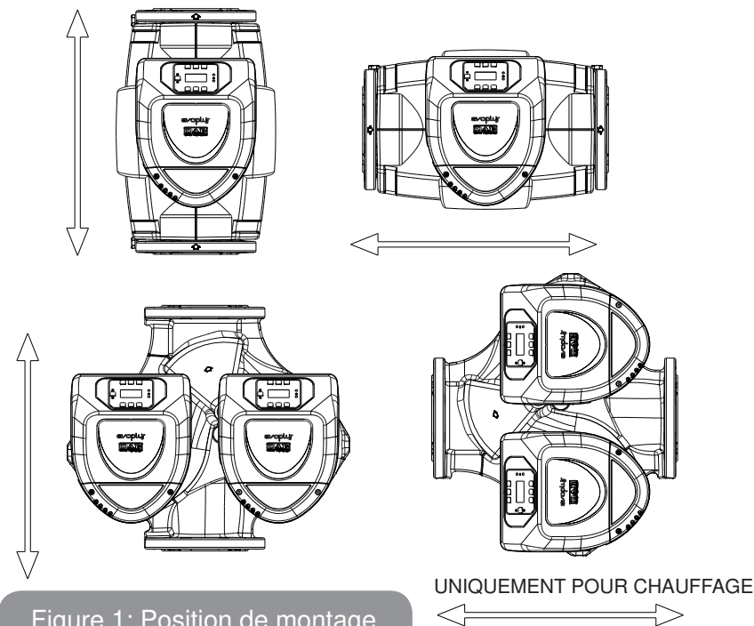
Figure 1: Position de montage
