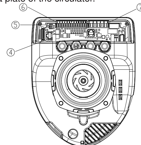
Figure 5: Electrical connections (rear)
