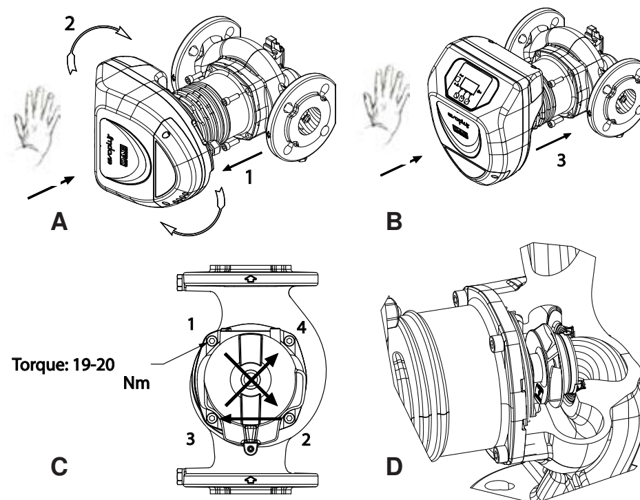
Figure 2: Instructions for motor head assembly
